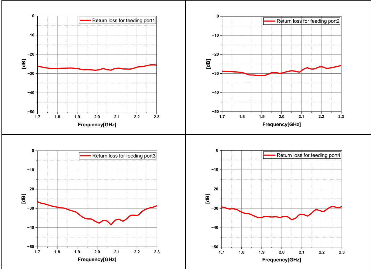
Typical Performance : 1700MHz to 2500MHz (Case 1)
