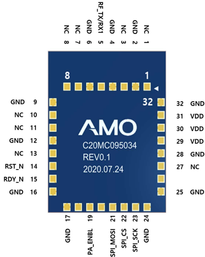
Figure 6 : Pinout Description(Bottom View)
