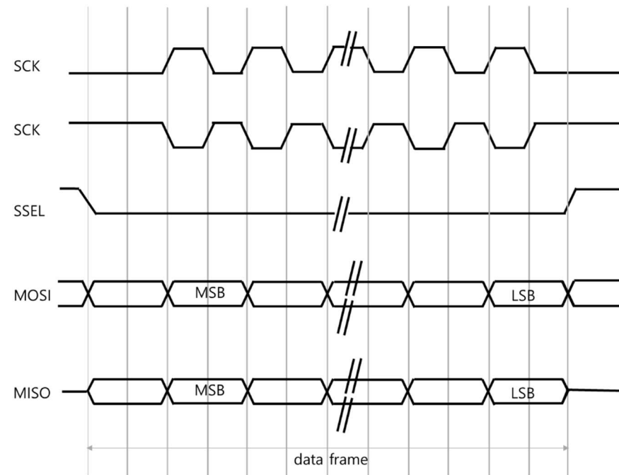
Figure 3. SPI date frame
