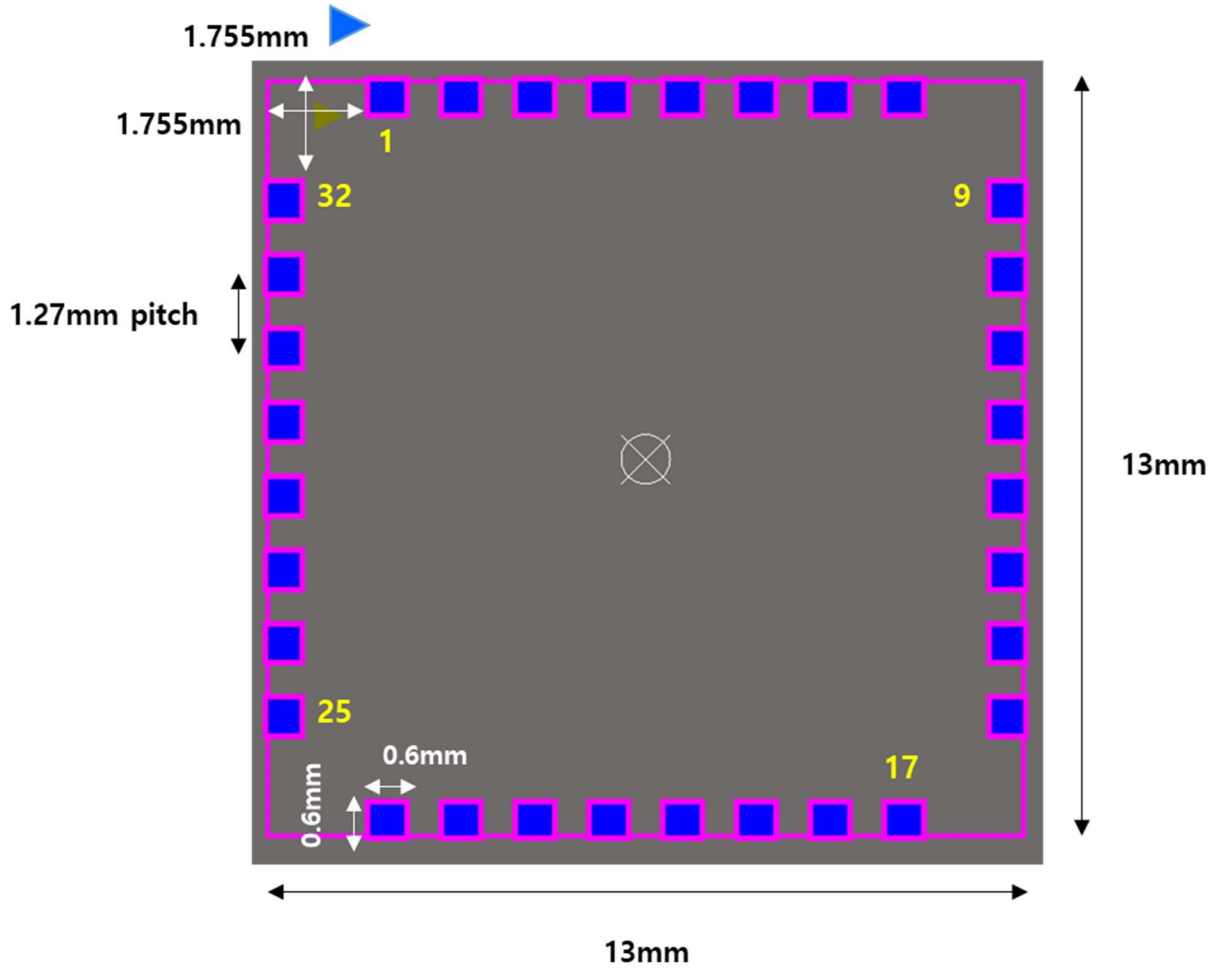
Figure 7. Pin Dimension or Footprint (TOP View)
