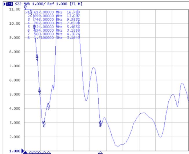
VSWR_ Middle
