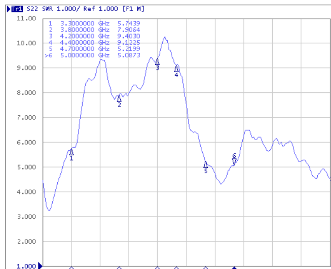
VSWR_ High
